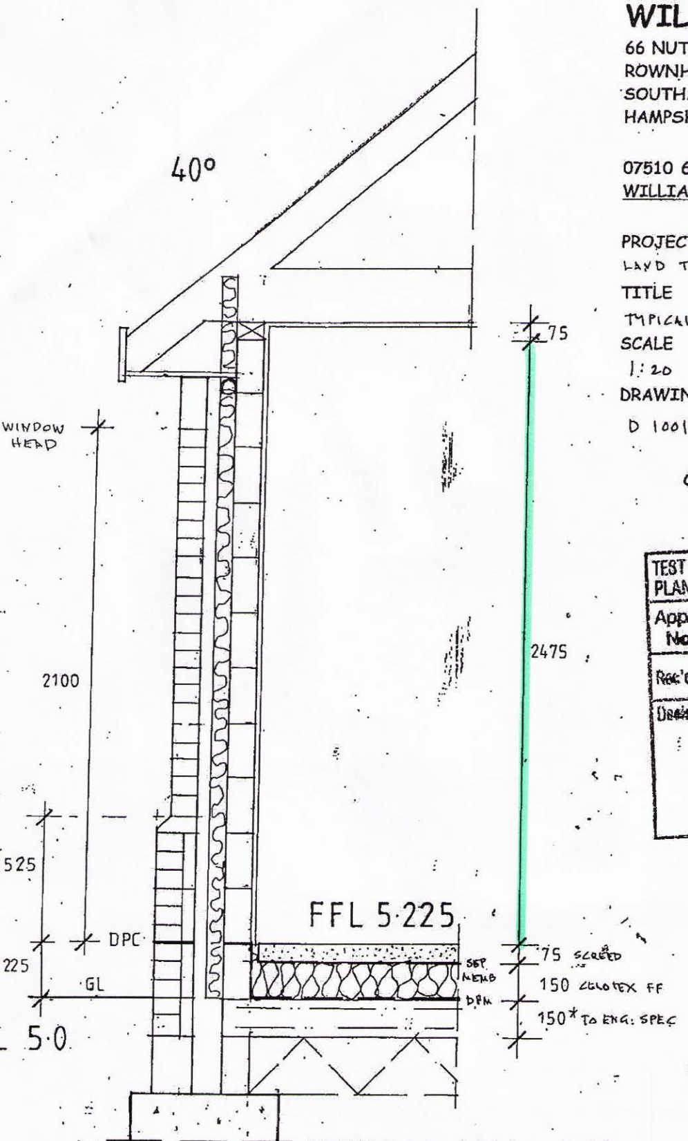
TYPICAL WALL 1:20
